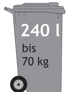
240 l bis 70 kg H = 107,6 cm B = 58,0 cm T = 73,0 cm
